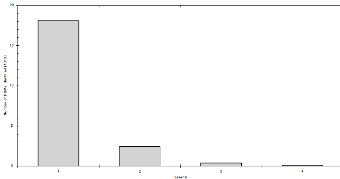
Figure 48. Number of PSMs identified in each round search.
