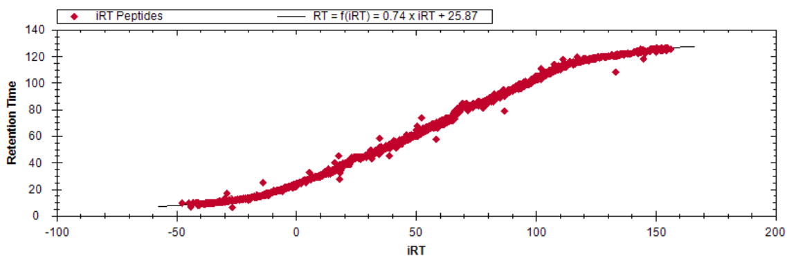
Figure 44. iRT calibration plot showing the non-linear transformation from iRT peptide repository to actual predicted retention times. The extended calibration allows you to correct even small gradient fine-structure fluctuations in order to get the most accurate retention time prediction for your run.
