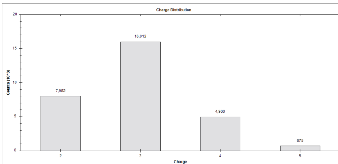
Figure 59. The Charge Distribution plot shows the number of peptide precursors with a given charge state across the entire experiment.
