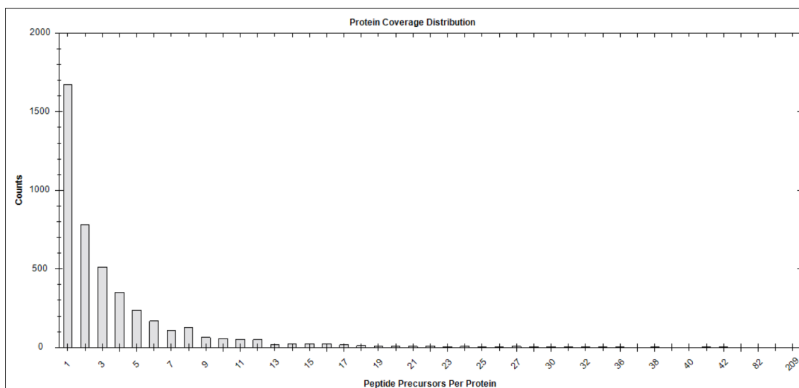
Figure 58. The protein Coverage shows distribution of numbers of precursors per protein.
