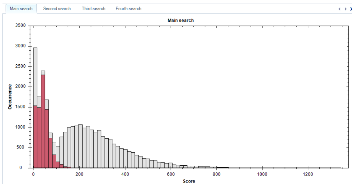
Figure 47. Behavior of the target (gray) and decoy (red) distributions for each of the round searches performed (in tabs).
