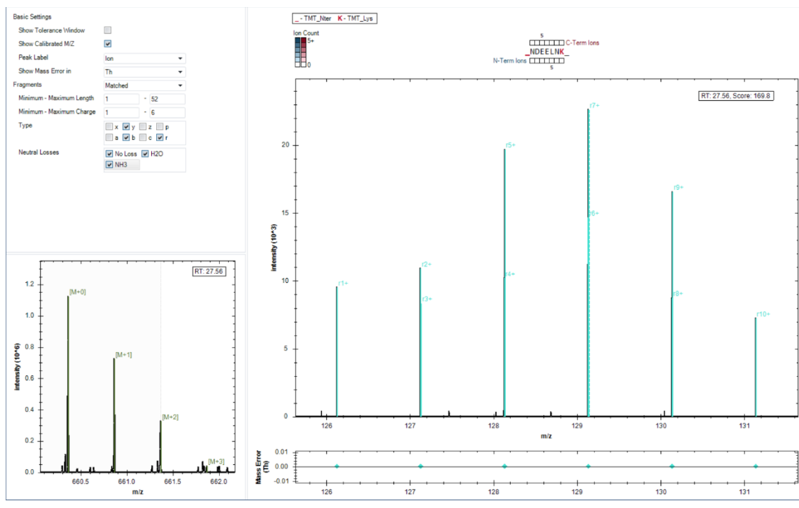
Figure 53. Corresponding MS3 spectrum. This plot shows the MS3 spectrum match, if applicable. In this example, the reporter ions for a TMT10-plex experiment can be nicely observed for a particular precursor.
